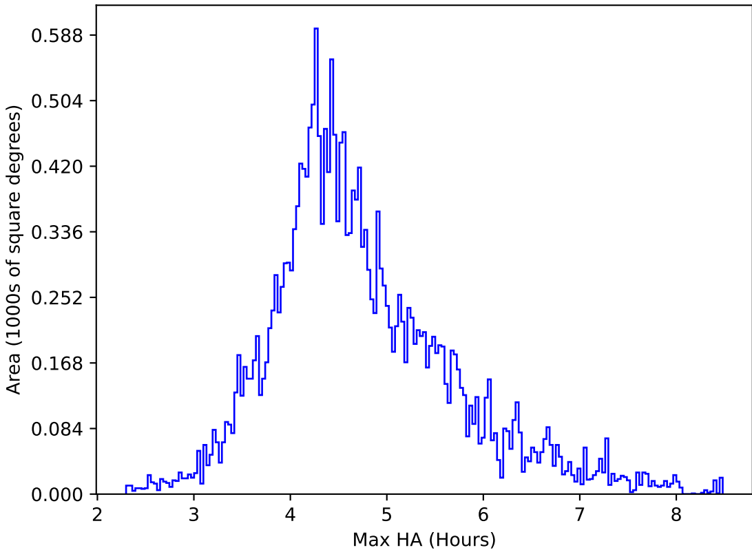
too_elab_r64_d3_gz_v3.4_10yrs All sky y band: Max HA
