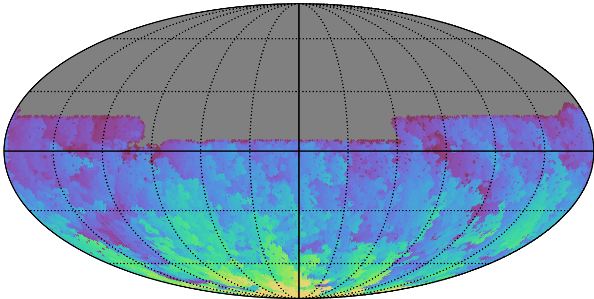
too_elab_r64_d3_gz_v3.4_10yrs All sky u band: Max HA
