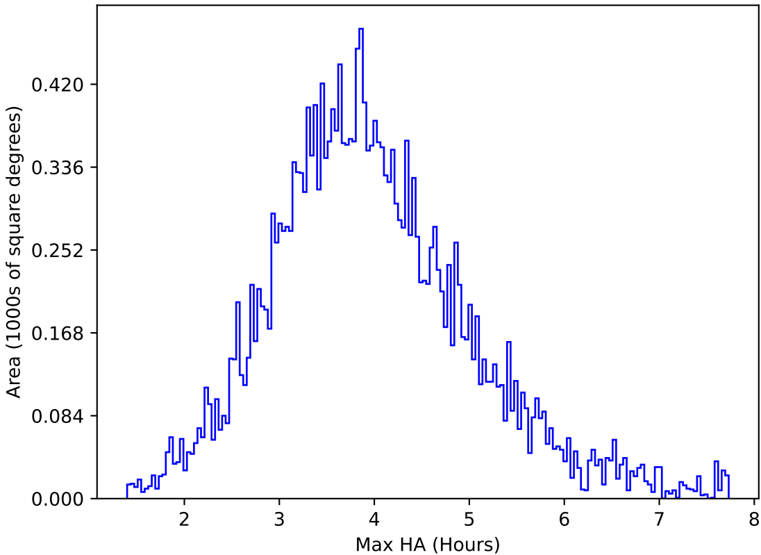
too_elab_r64_d3_gz_v3.4_10yrs All sky u band: Max HA
