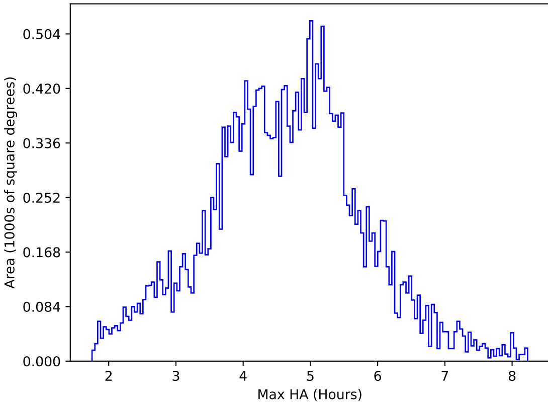
too_elab_r64_d3_gz_v3.4_10yrs All sky i band: Max HA
