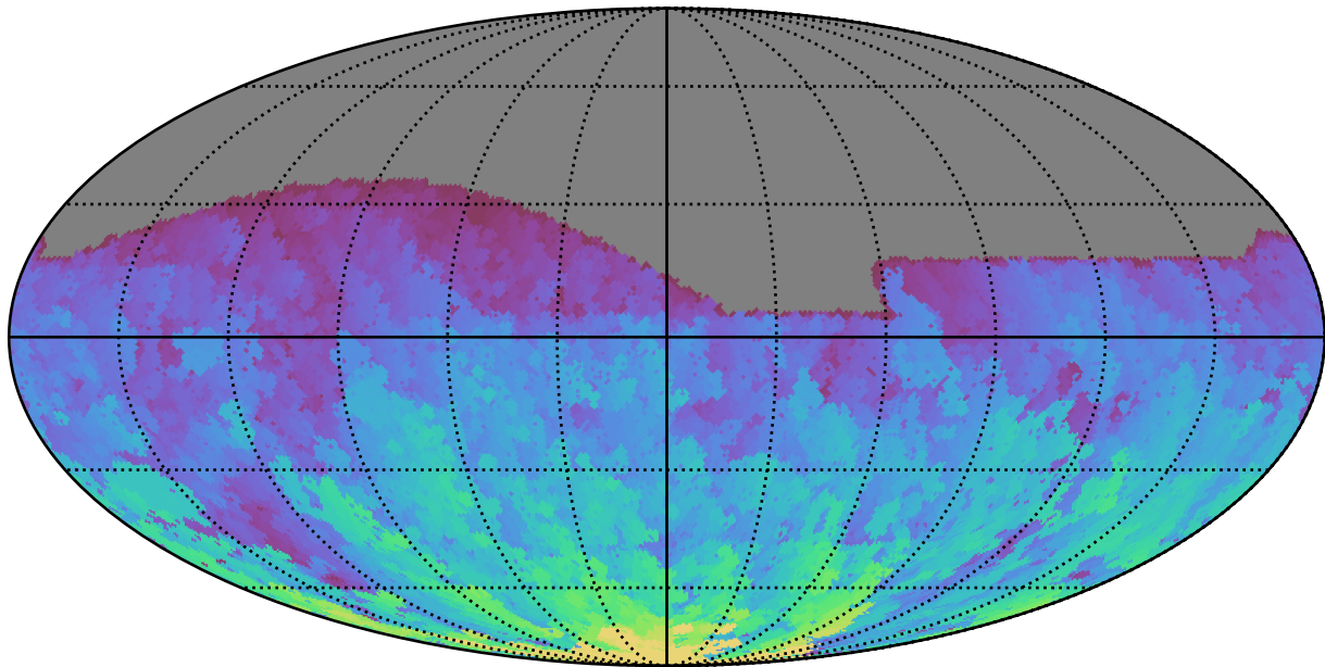
too_elab_r64_d3_gz_v3.4_10yrs All sky g band: Max HA
