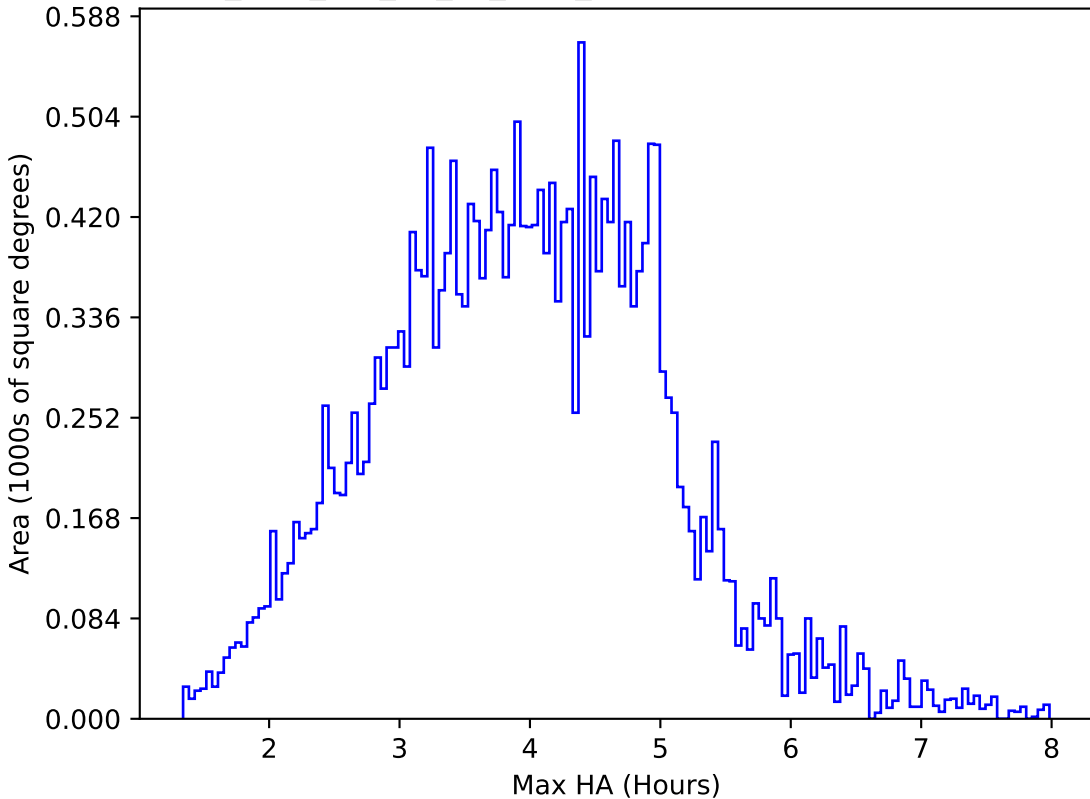
too_elab_r64_d3_gz_v3.4_10yrs All sky g band: Max HA
