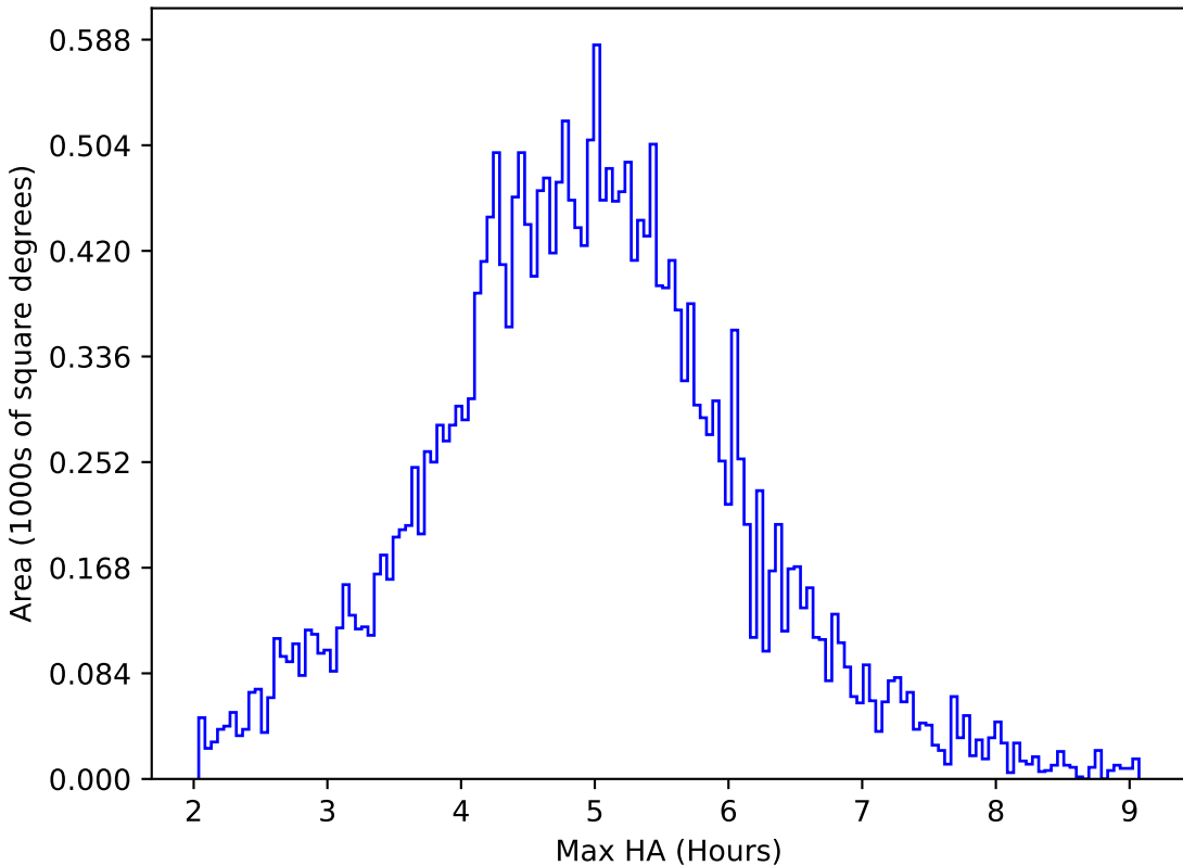
too_elab_r64_d3_gz_v3.4_10yrs All sky all bands: Max HA
