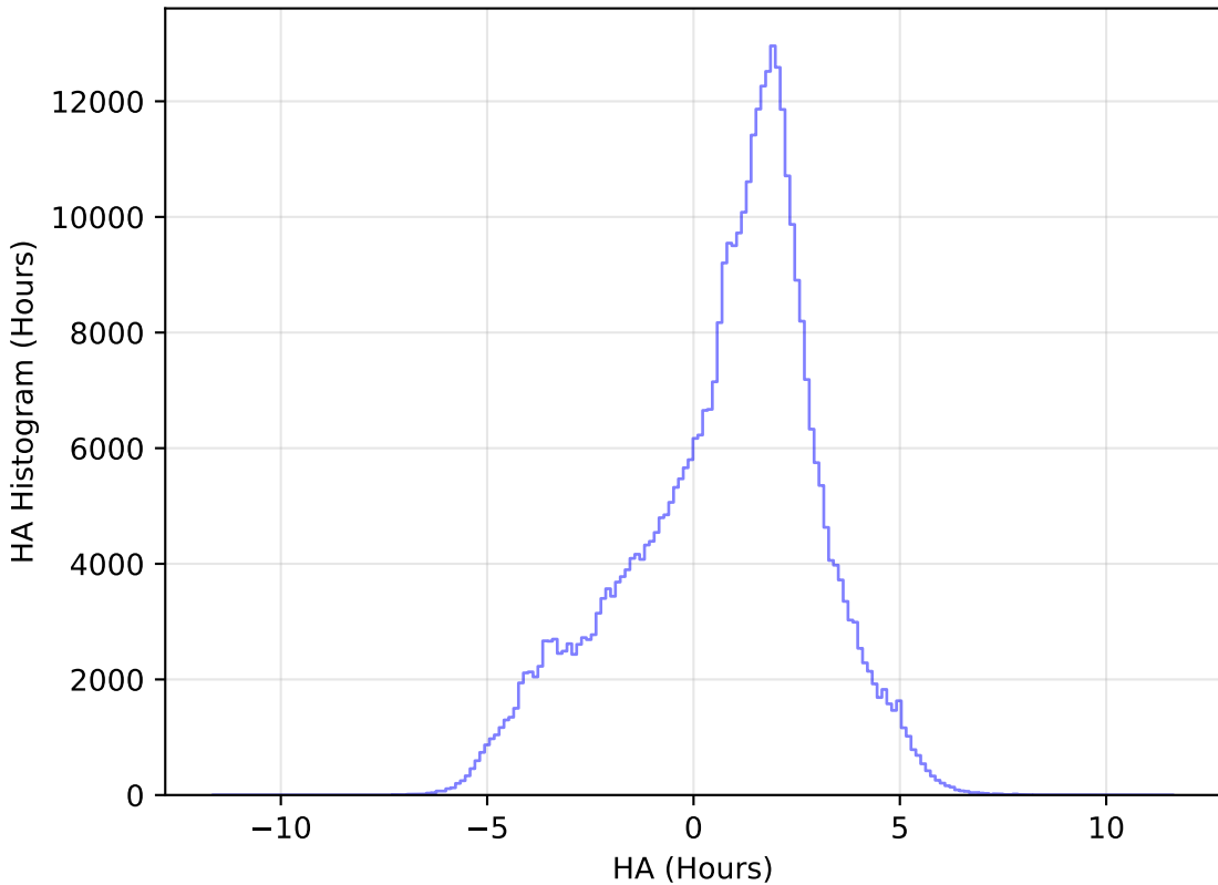
too_elab_r64_d3_gz_v3.4_10yrs WFD z band: HA Histogram
