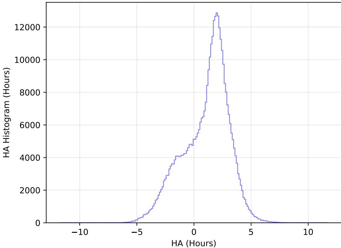
too_elab_r64_d3_gz_v3.4_10yrs WFD y band: HA Histogram
