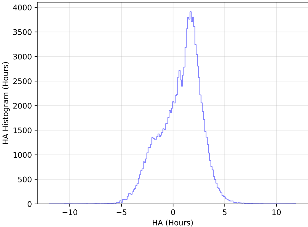
too_elab_r64_d3_gz_v3.4_10yrs WFD u band: HA Histogram
