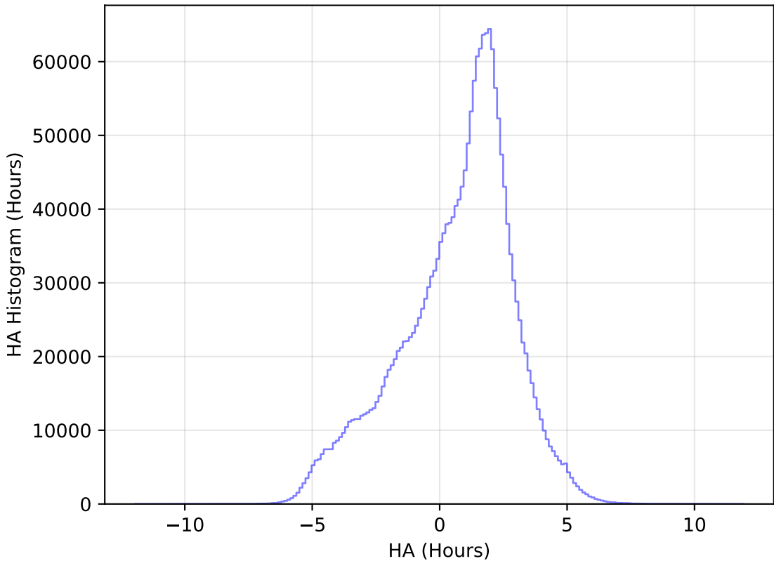
too_elab_r64_d3_gz_v3.4_10yrs WFD all bands: HA Histogram
