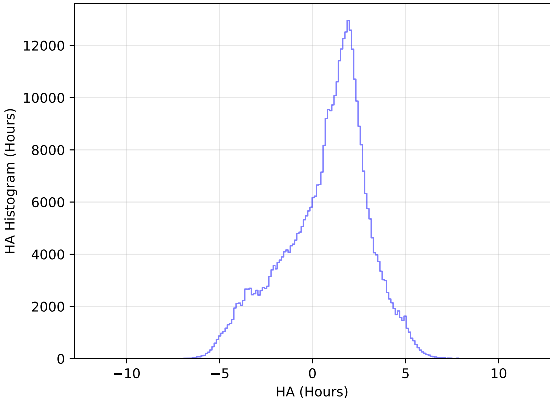
too_elab_r64_d3_gz_v3.4_10yrs All sky z band: HA Histogram
