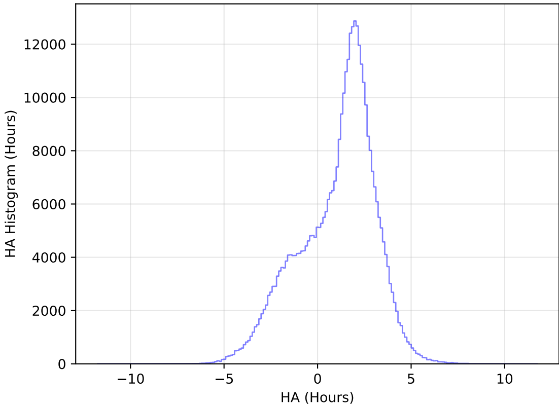
too_elab_r64_d3_gz_v3.4_10yrs All sky y band: HA Histogram
