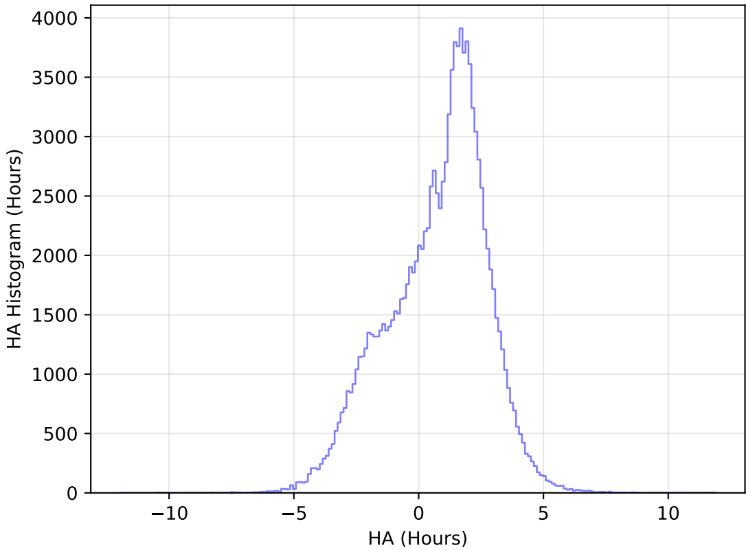
too_elab_r64_d3_gz_v3.4_10yrs All sky u band: HA Histogram
