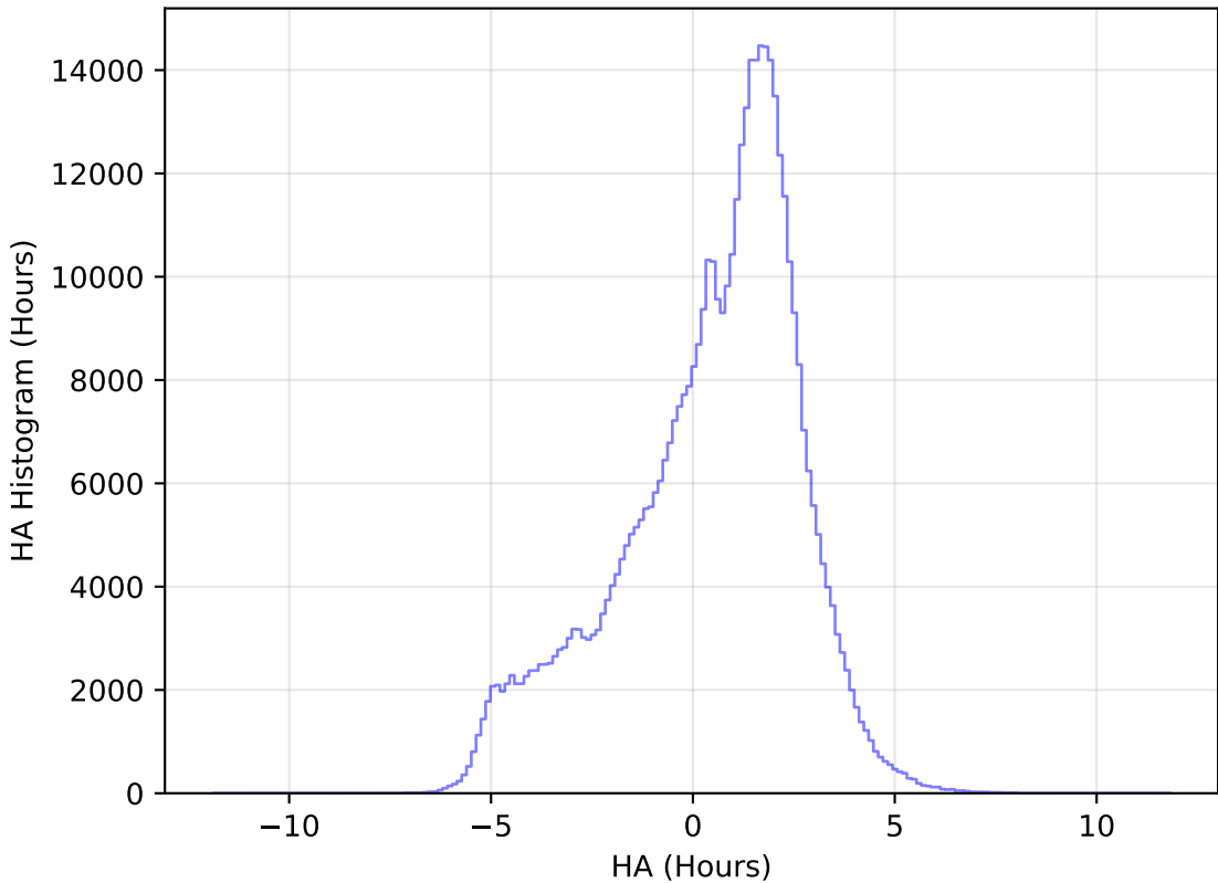
too_elab_r64_d3_gz_v3.4_10yrs All sky r band: HA Histogram
