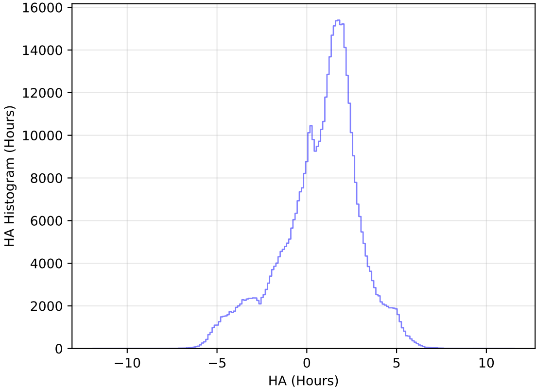
too_elab_r64_d3_gz_v3.4_10yrs All sky i band: HA Histogram
