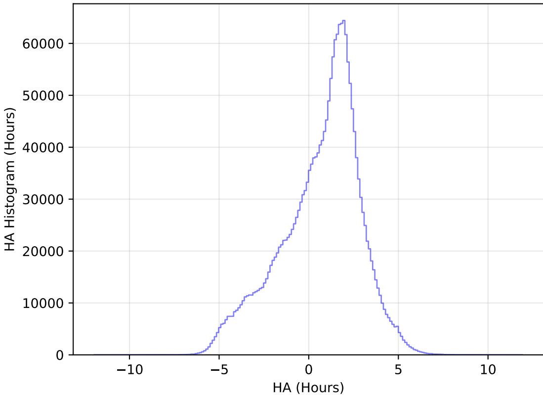
too_elab_r64_d3_gz_v3.4_10yrs All sky all bands: HA Histogram
