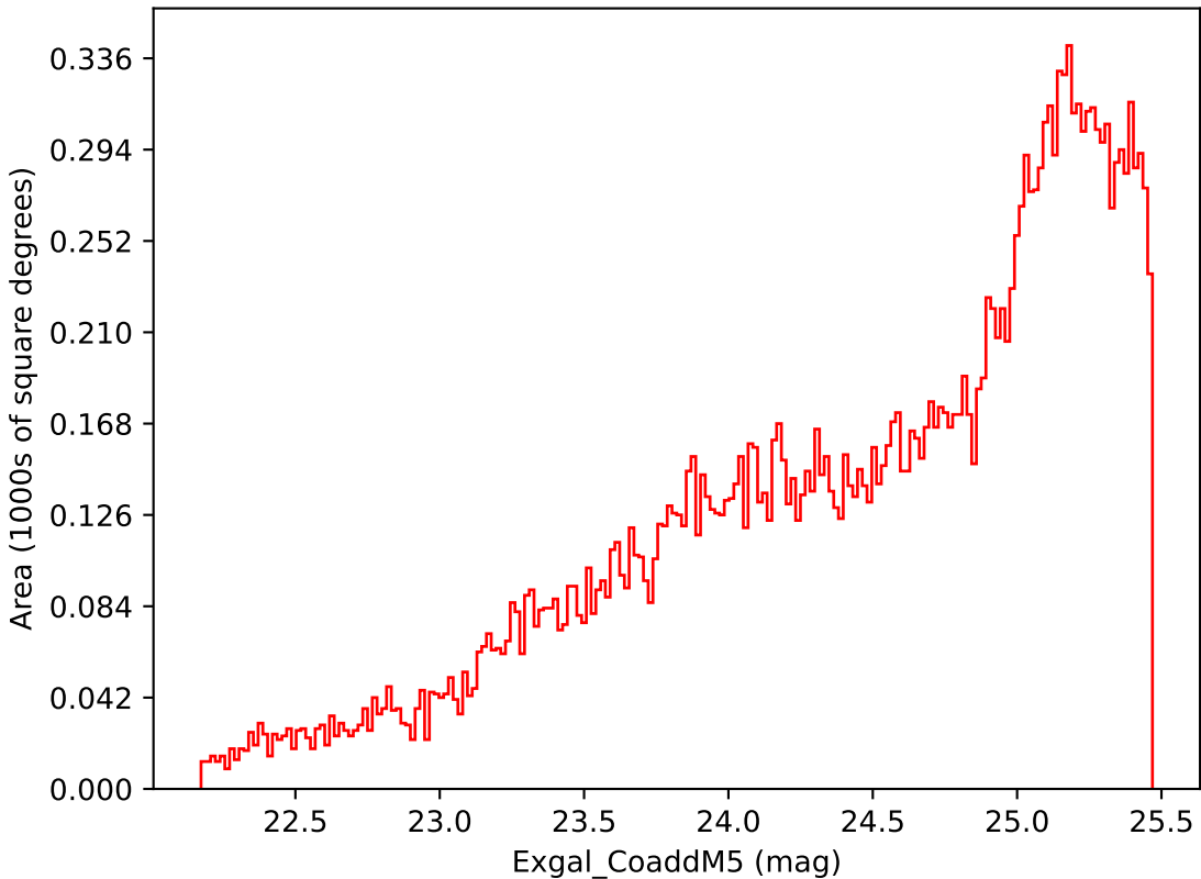
too_elab_r64_d3_gz_v3.4_10yrs Yr 3-4 i band: Exgal_CoaddM5
