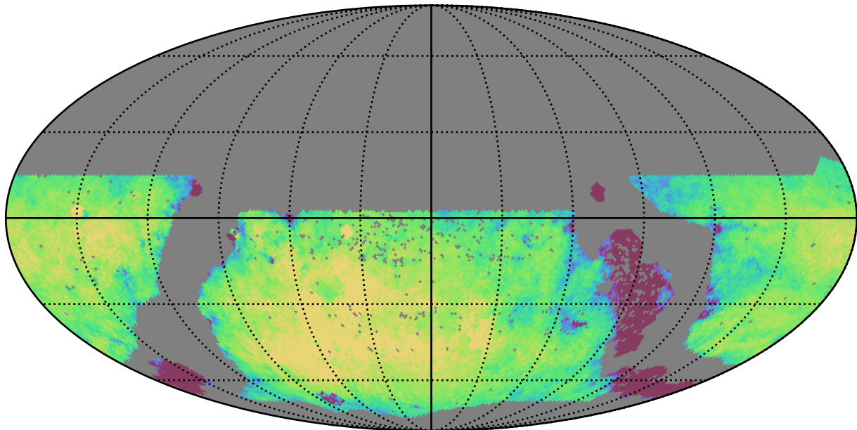
too_elab_r64_d3_gz_v3.4_10yrs WFD g band: Exgal_CoaddM5
