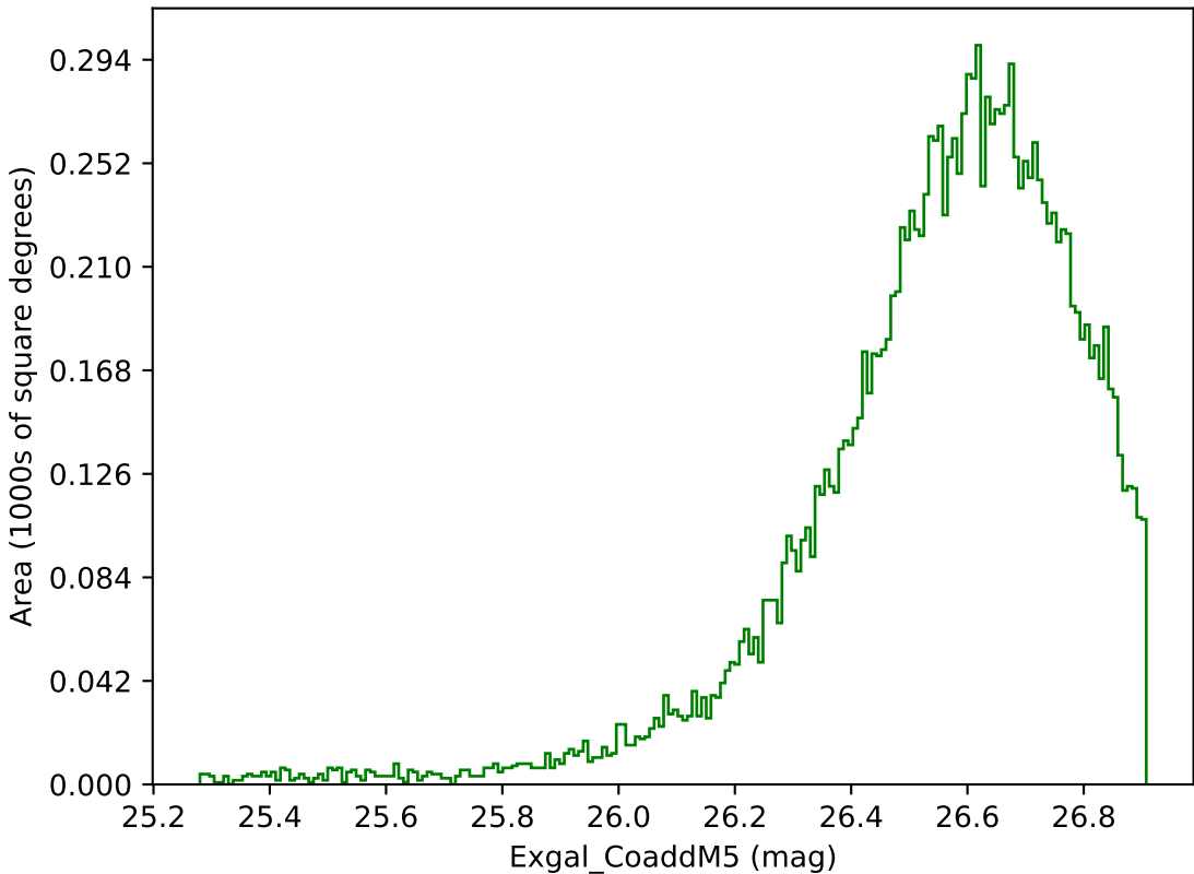
too_elab_r64_d3_gz_v3.4_10yrs WFD g band: Exgal_CoaddM5
