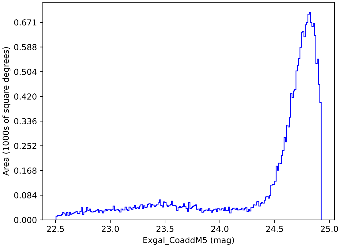
too_elab_r64_d3_gz_v3.4_10yrs All sky y band: Exgal_CoaddM5
