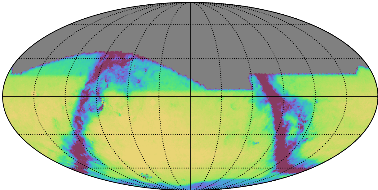
too_elab_r64_d3_gz_v3.4_10yrs All sky r band: Exgal_CoaddM5
