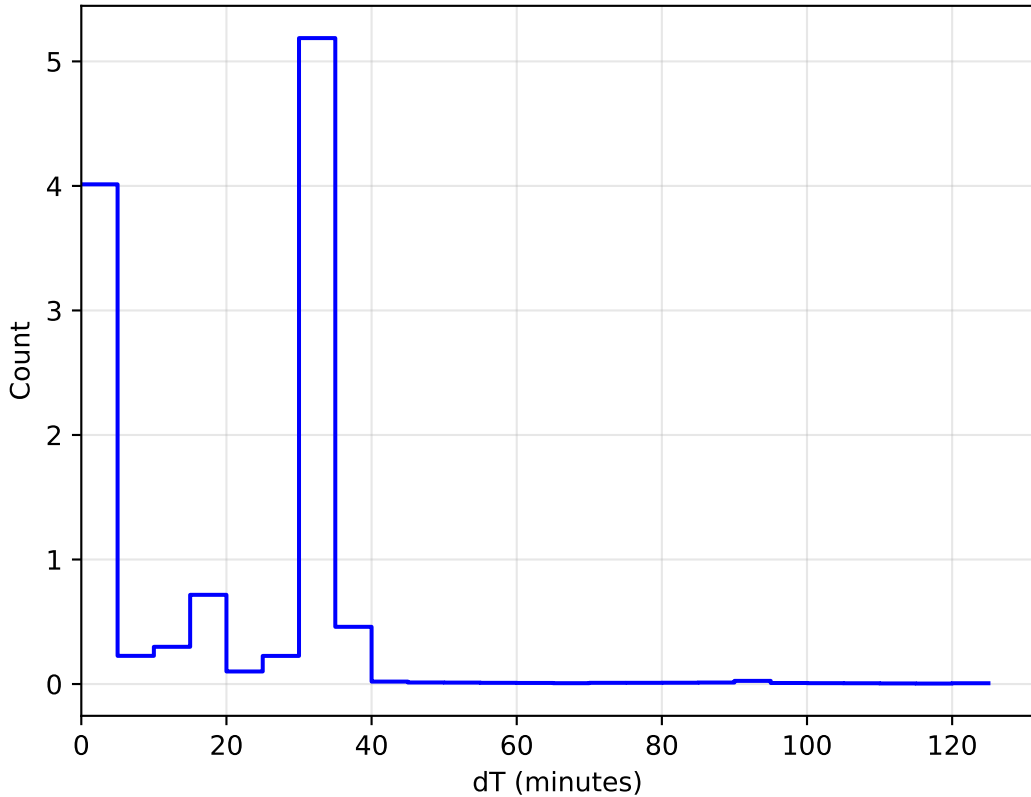
too_elab_r64_d3_gz_v3.4_10yrs WFD: DeltaT Histogram
