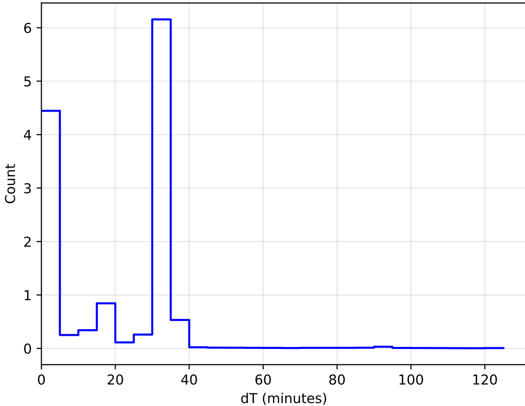
too_elab_r64_d3_gz_v3.4_10yrs All sky: DeltaT Histogram 1e6
