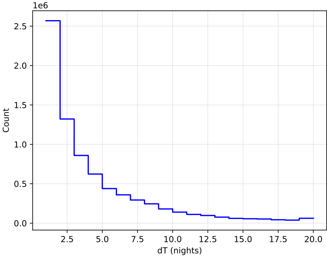
too_elab_r64_d3_gz_v3.4_10yrs WFD all bands: DeltaNight Histogram
