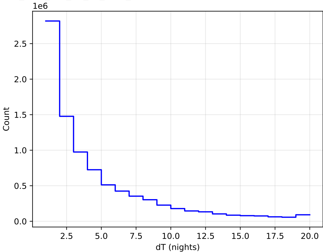
too_elab_r64_d3_gz_v3.4_10yrs All sky all bands: DeltaNight Histogram
