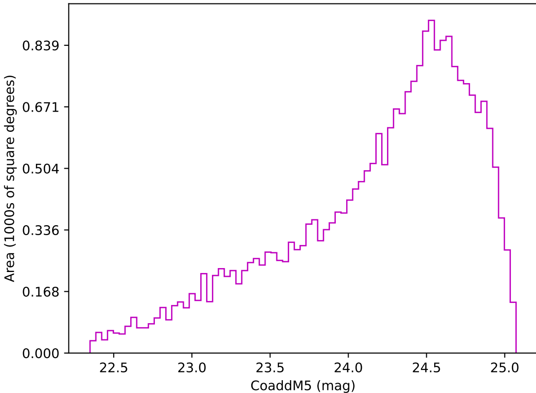
too_elab_r64_d3_gz_v3.4_10yrs Yr 3-4 z band: CoaddM5
