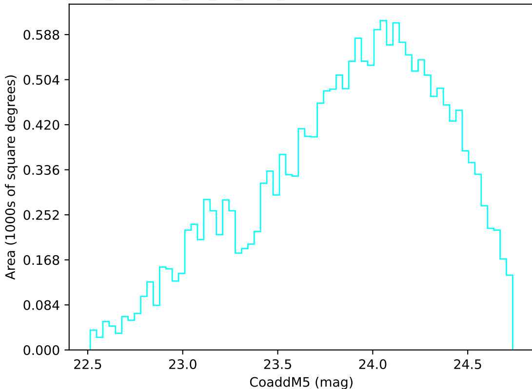
too_elab_r64_d3_gz_v3.4_10yrs Yr 3-4 u band: CoaddM5
