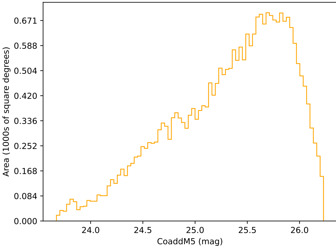
too_elab_r64_d3_gz_v3.4_10yrs Yr 3-4 r band: CoaddM5
