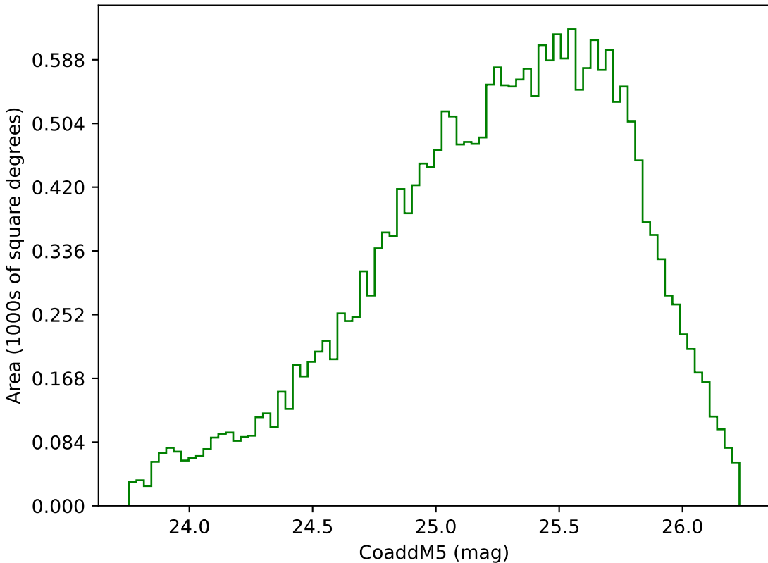
too_elab_r64_d3_gz_v3.4_10yrs Yr 3-4 g band: CoaddM5
