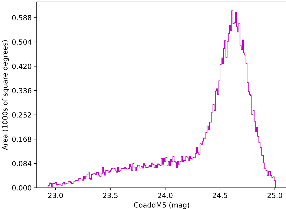
too_elab_r64_d3_gz_v3.4_10yrs Yr 1 z band: CoaddM5
