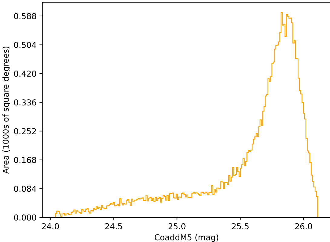
too_elab_r64_d3_gz_v3.4_10yrs Yr 1 r band: CoaddM5
