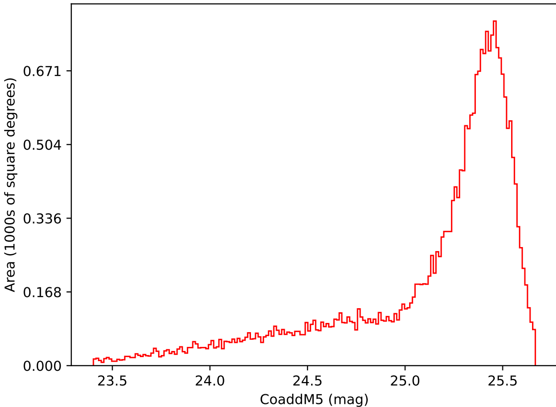
too_elab_r64_d3_gz_v3.4_10yrs Yr 1 i band: CoaddM5
