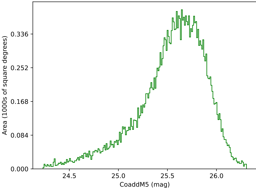
too_elab_r64_d3_gz_v3.4_10yrs Yr 1 g band: CoaddM5
