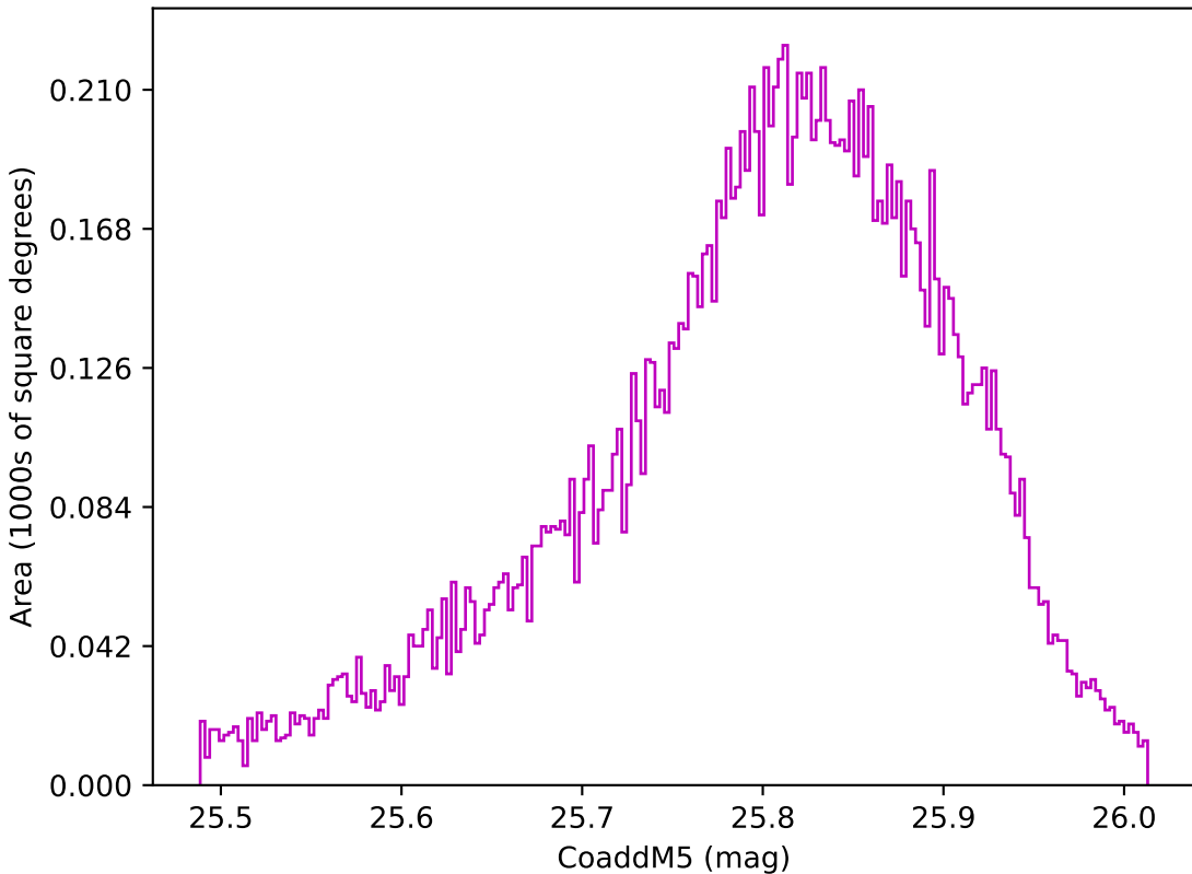
too_elab_r64_d3_gz_v3.4_10yrs WFD z band: CoaddM5
