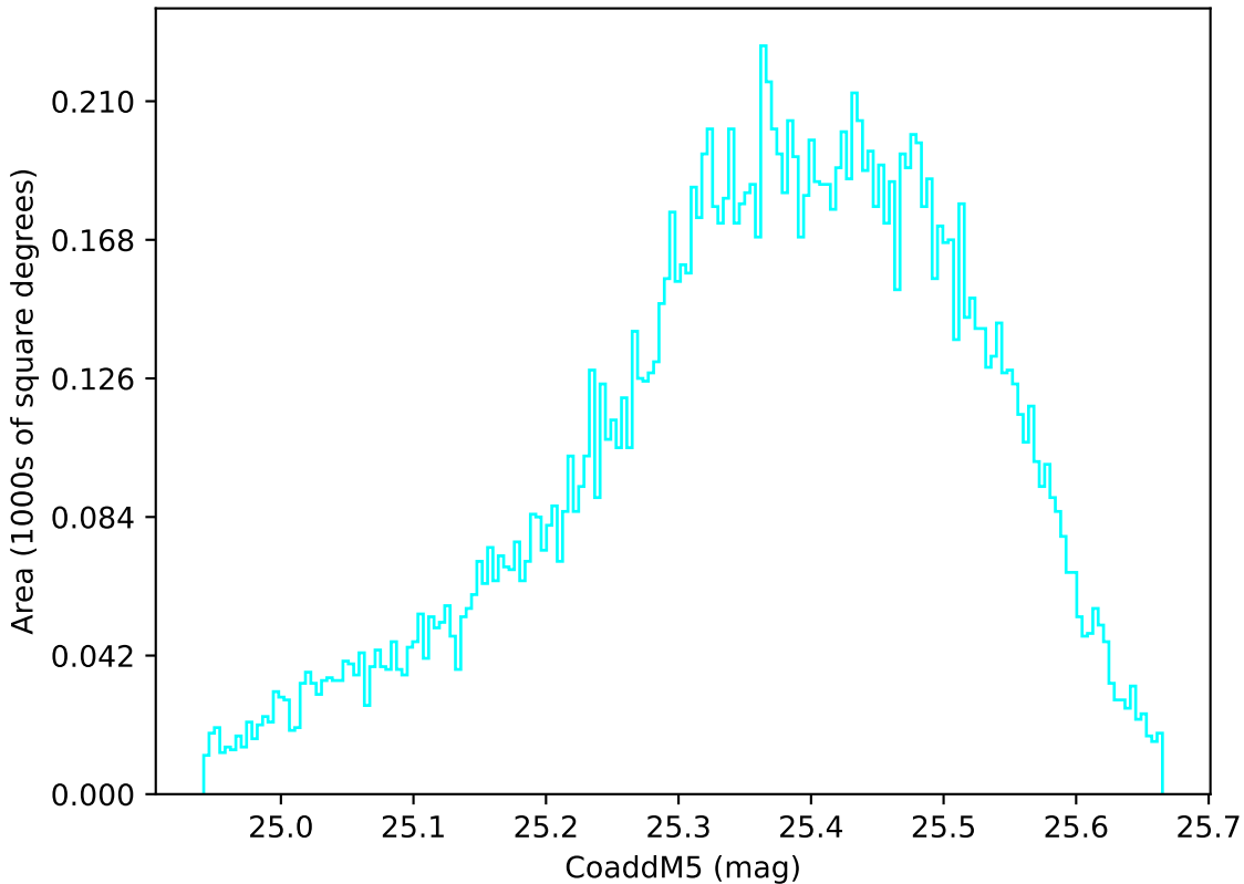
too_elab_r64_d3_gz_v3.4_10yrs WFD u band: CoaddM5
