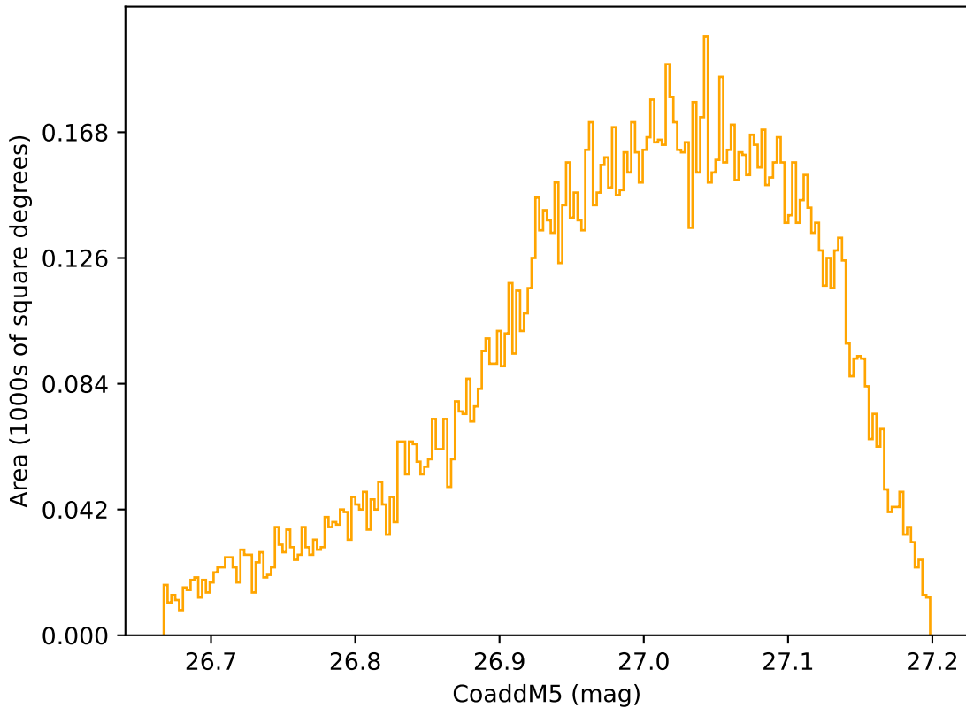
too_elab_r64_d3_gz_v3.4_10yrs WFD r band: CoaddM5
