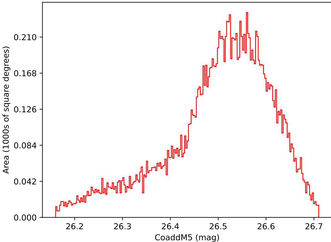
too_elab_r64_d3_gz_v3.4_10yrs WFD i band: CoaddM5
