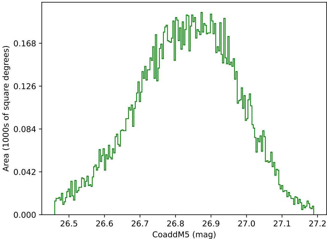
too_elab_r64_d3_gz_v3.4_10yrs WFD g band: CoaddM5
