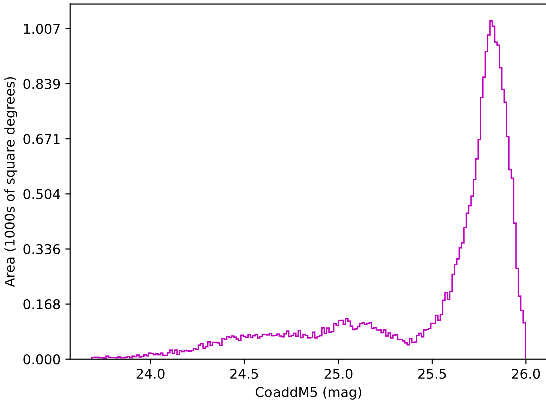
too_elab_r64_d3_gz_v3.4_10yrs All sky z band: CoaddM5
