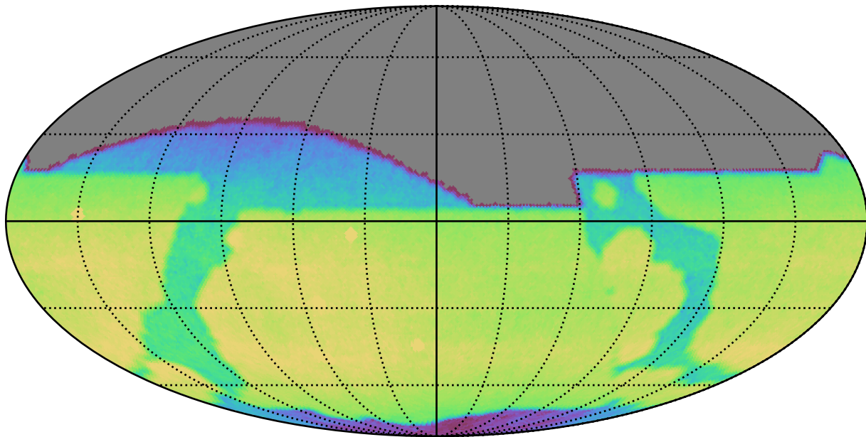
too_elab_r64_d3_gz_v3.4_10yrs All sky r band: CoaddM5
