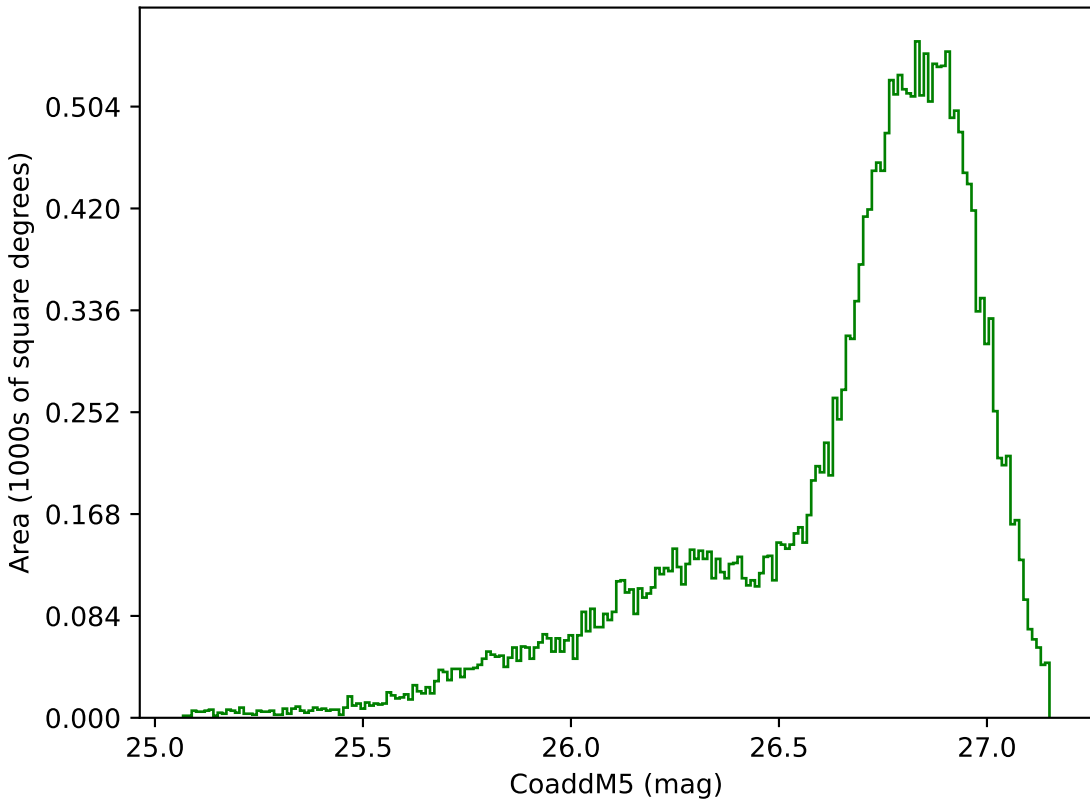
too_elab_r64_d3_gz_v3.4_10yrs All sky g band: CoaddM5
