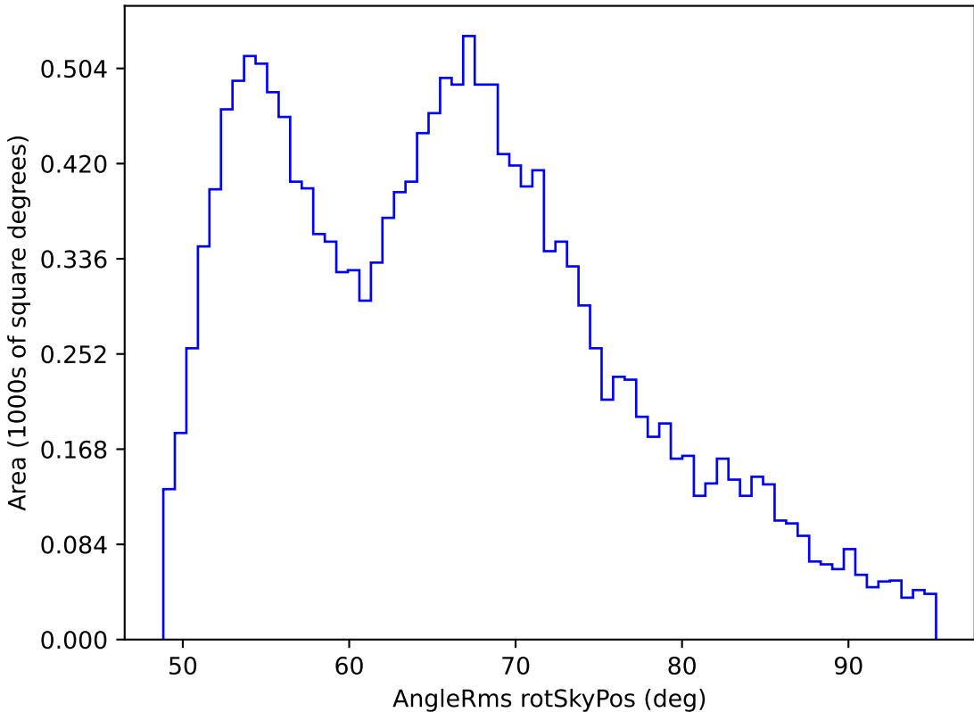
too_elab_r64_d3_gz_v3.4_10yrs WFD z band: AngleRms rotSkyPos
