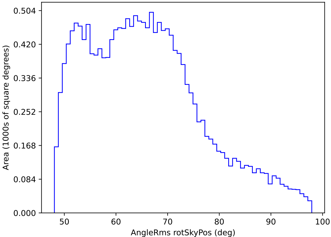
too_elab_r64_d3_gz_v3.4_10yrs WFD r band: AngleRms rotSkyPos
