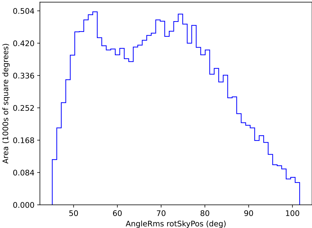
too_elab_r64_d3_gz_v3.4_10yrs WFD g band: AngleRms rotSkyPos
