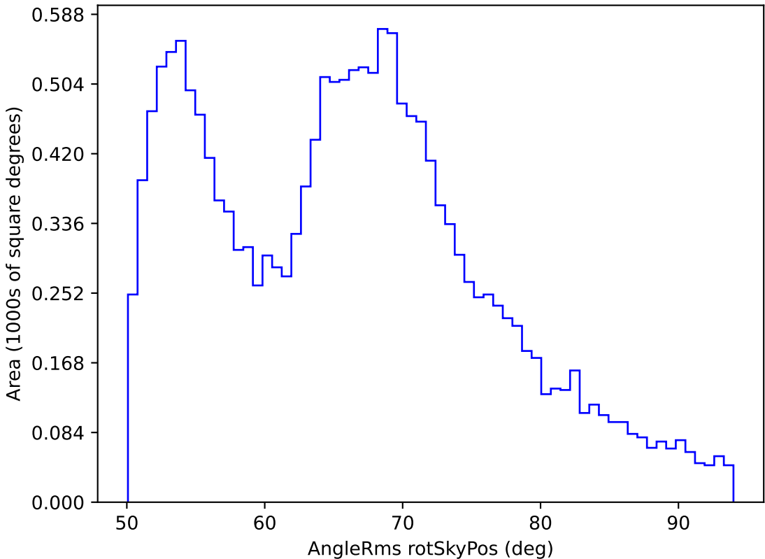
too_elab_r64_d3_gz_v3.4_10yrs WFD all bands: AngleRms rotSkyPos
