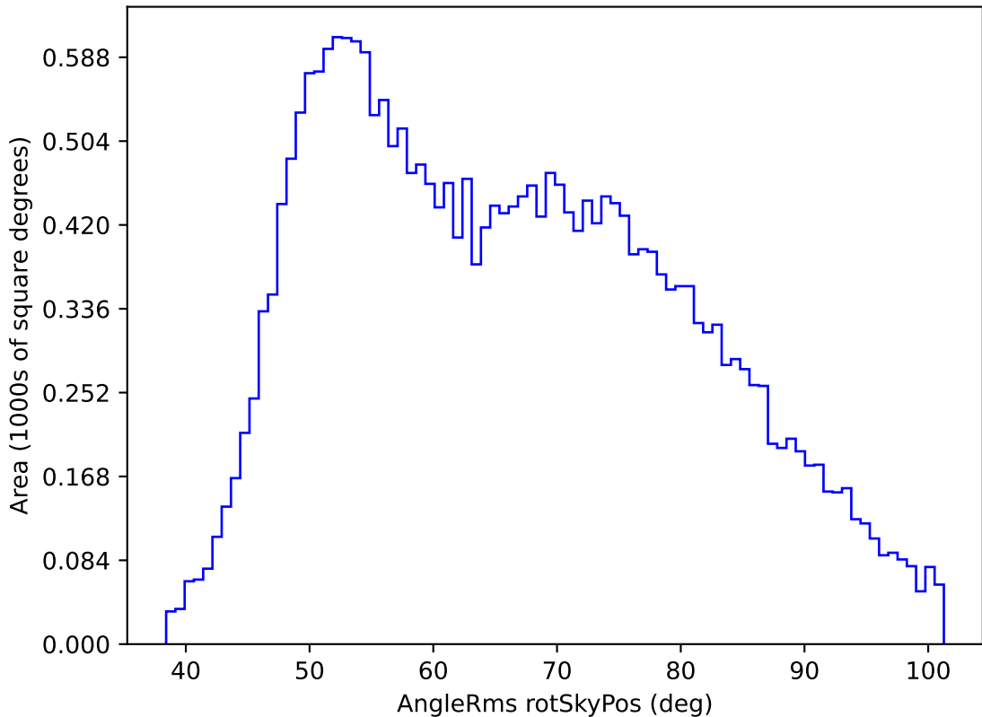
too_elab_r64_d3_gz_v3.4_10yrs All sky g band: AngleRms rotSkyPos
