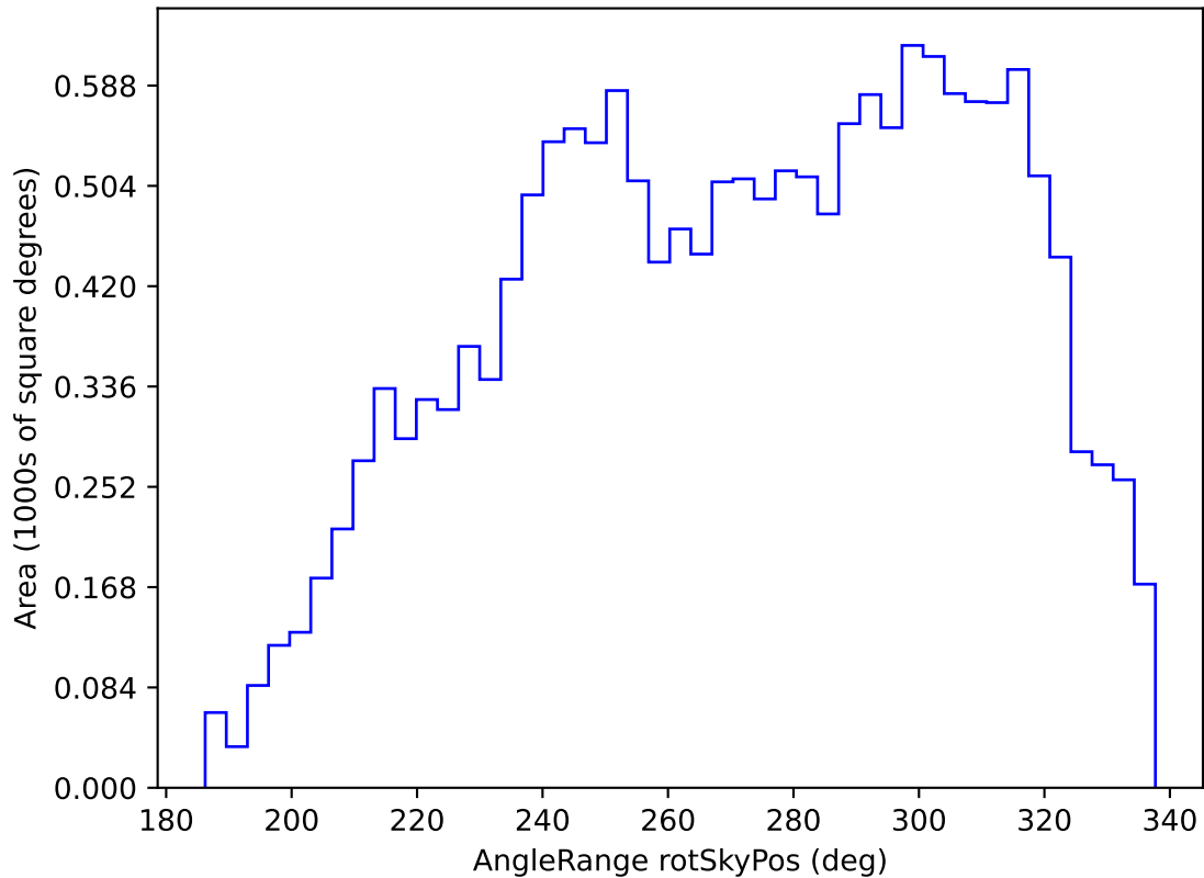
too_elab_r64_d3_gz_v3.4_10yrs WFD y band: AngleRange rotSkyPos
