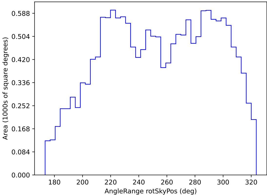
too_elab_r64_d3_gz_v3.4_10yrs WFD u band: AngleRange rotSkyPos
