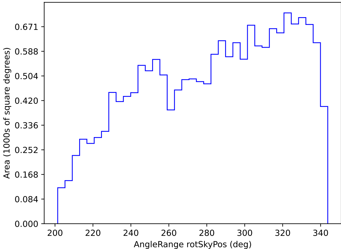
too_elab_r64_d3_gz_v3.4_10yrs WFD r band: AngleRange rotSkyPos
